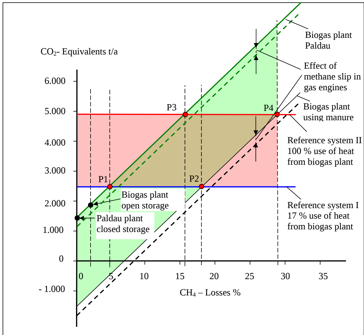
Figure 4.13: CO 2 -eq emissions versus CH 4 losses.
